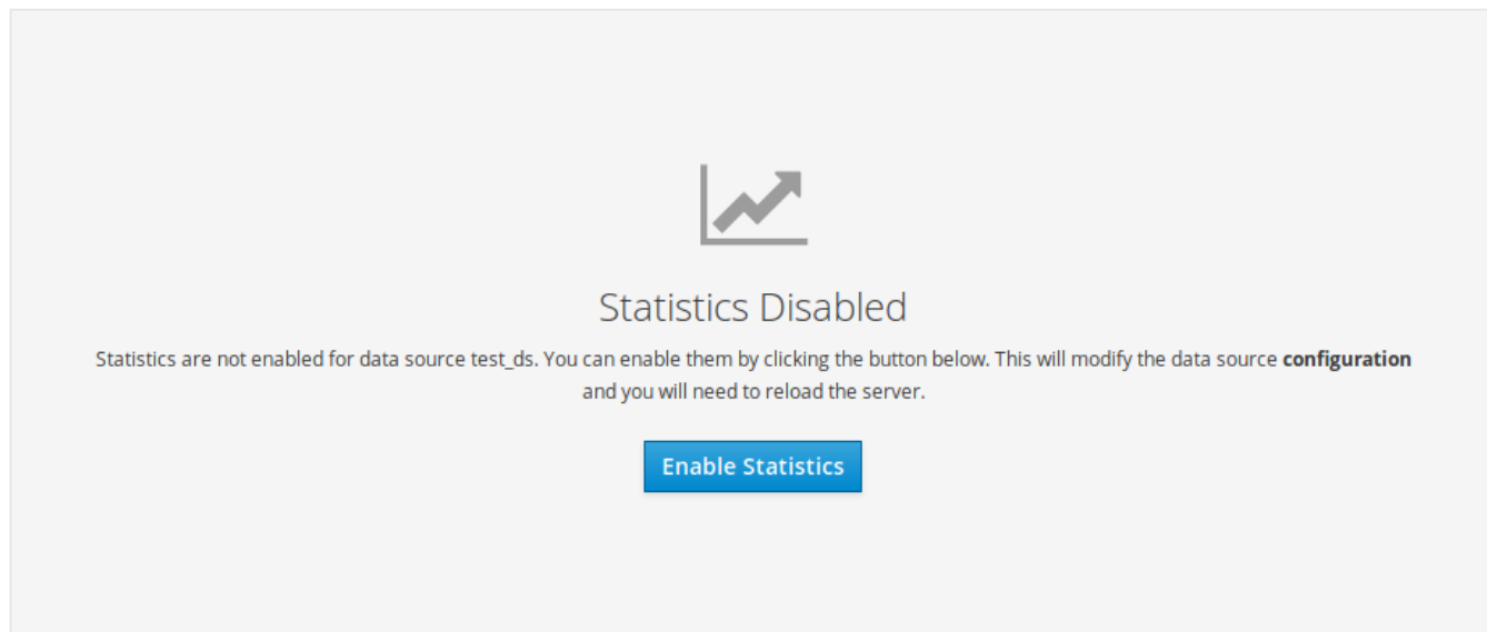
Figure 7.10: Enable statistics
