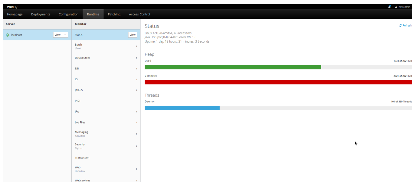
Figure 7.11: Память
