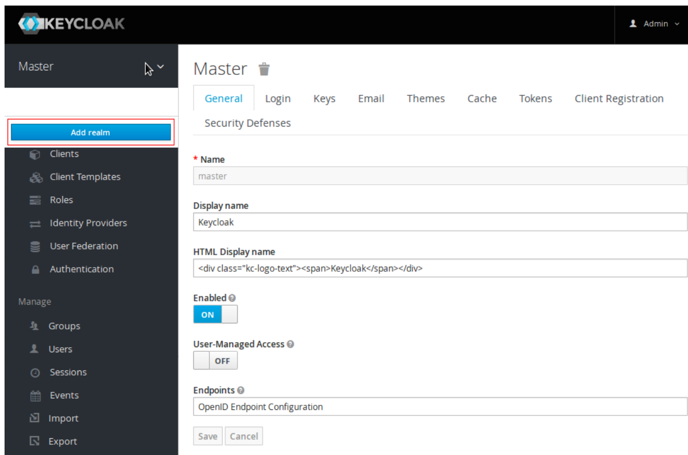
Figure 7.55: Add Realm
