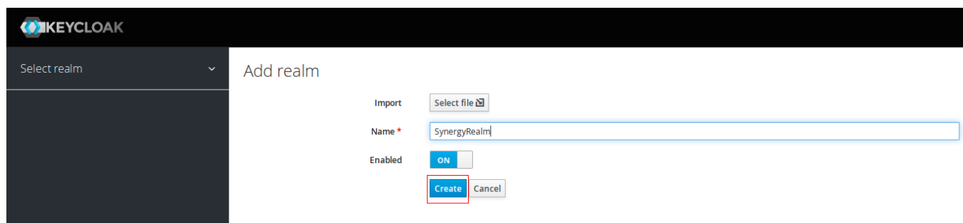
Figure 7.56: Synergy Realm
