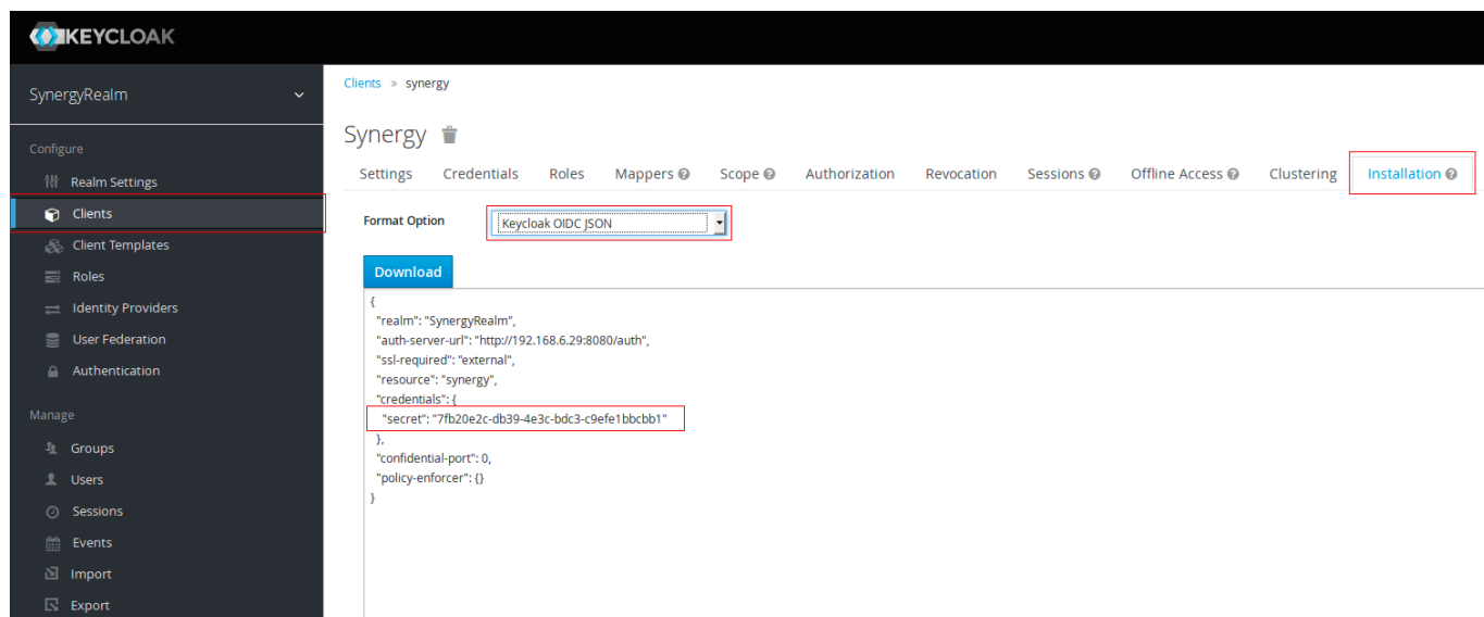
Figure 7.63: Поле secret
