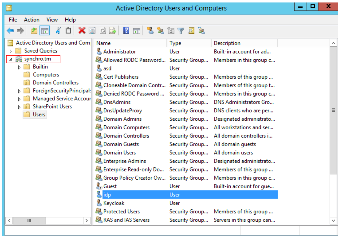
Figure 7.48: Active Directory
