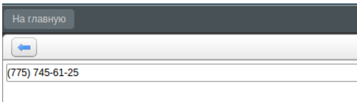
Figure 3.44: Input mask in fill mode
